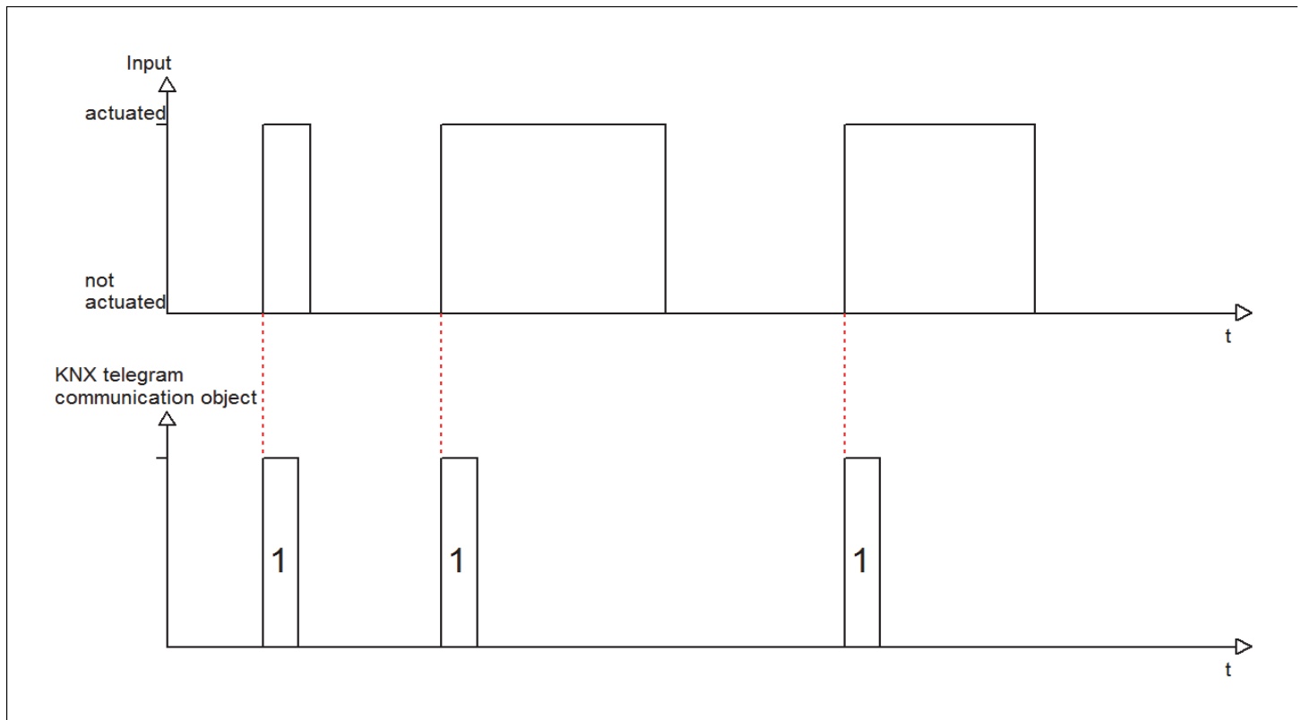
Picture 10: Press to send on signal
