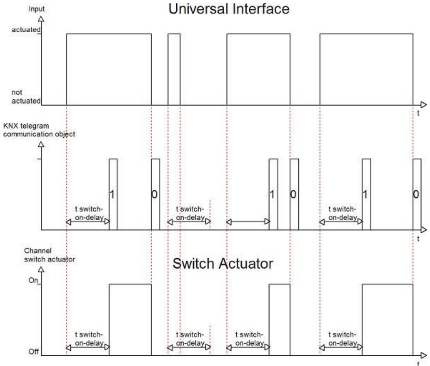
picture 15: Delayed transmission
