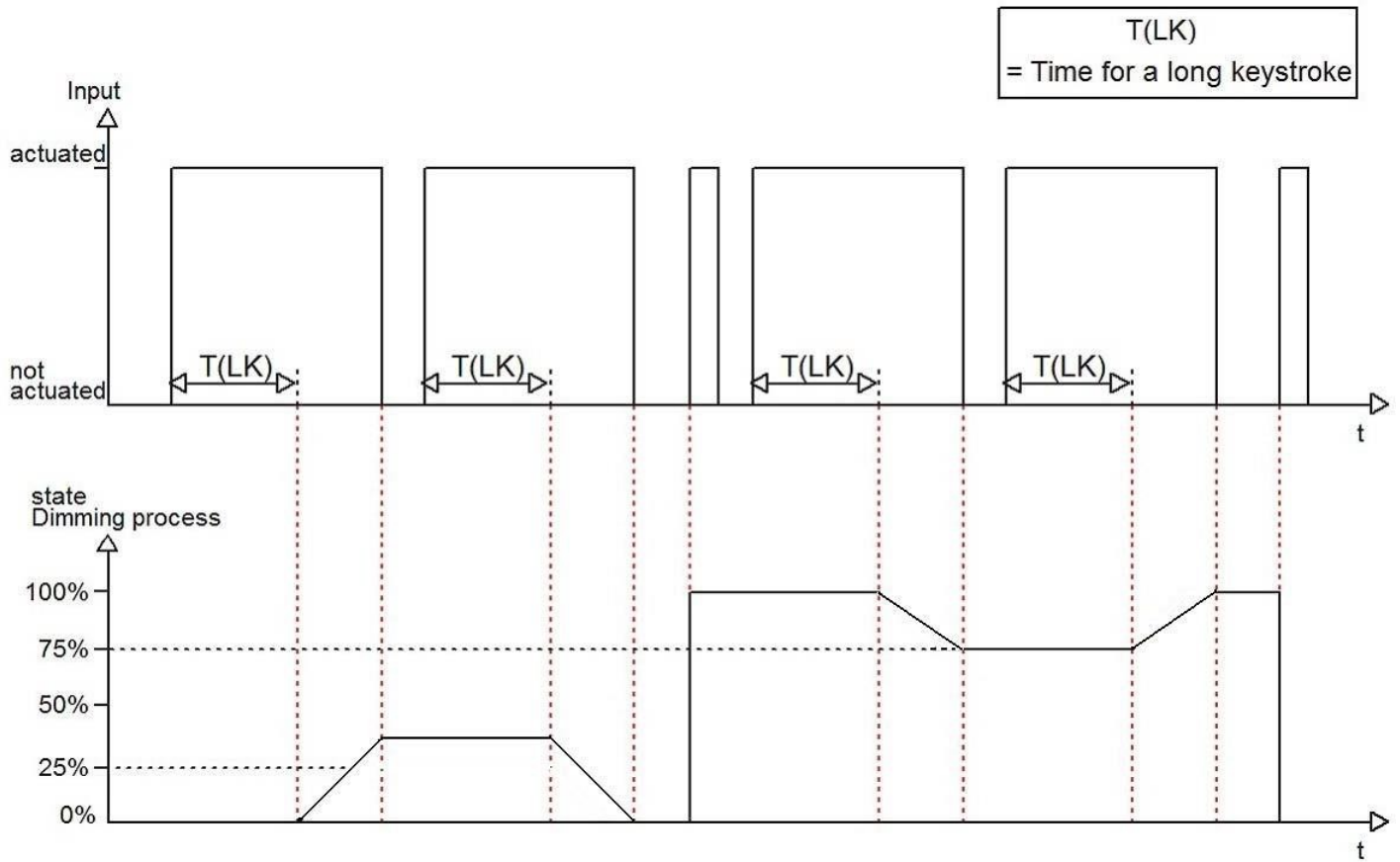
Picture 24: one button dimming
