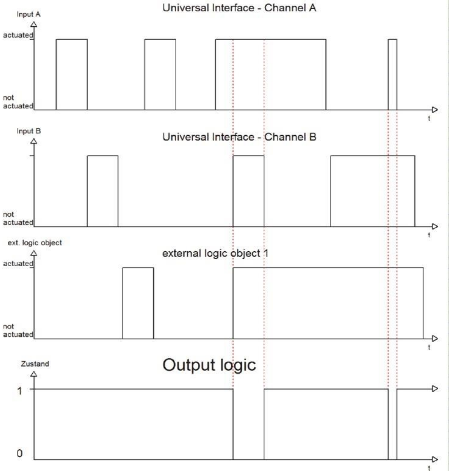
Picture 29: Logical output
