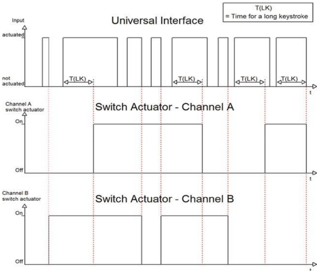
Picture 21: Long press / short press are independent
