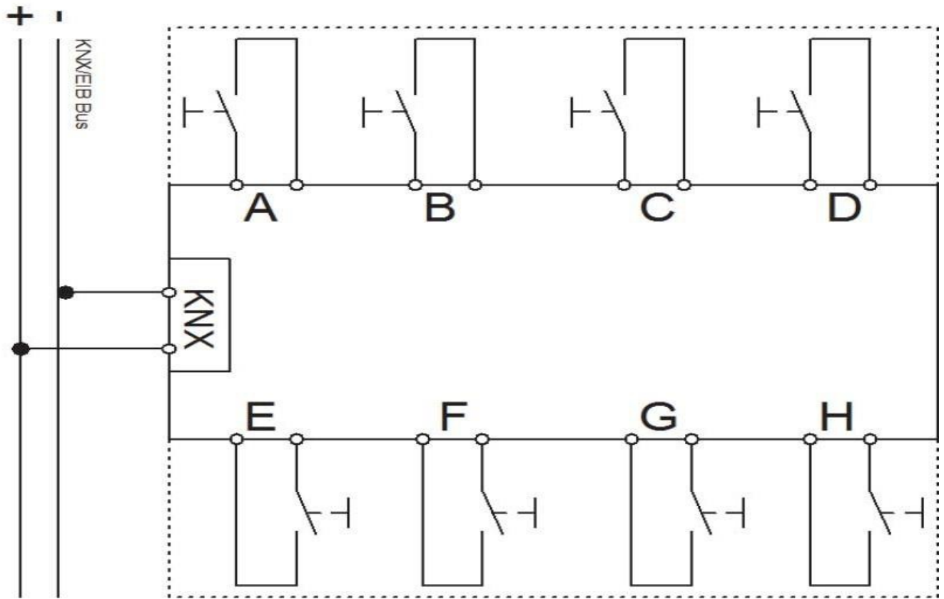
Picture1: Wiring diagram,8-Channel push button
