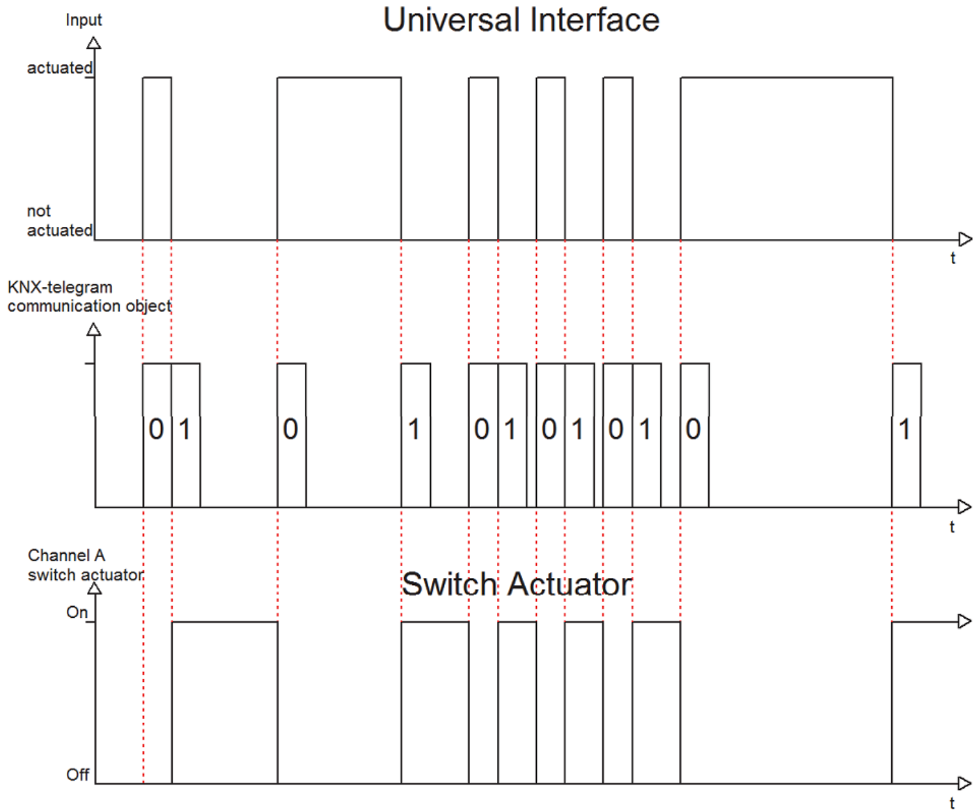
Picture 13: Send status value
