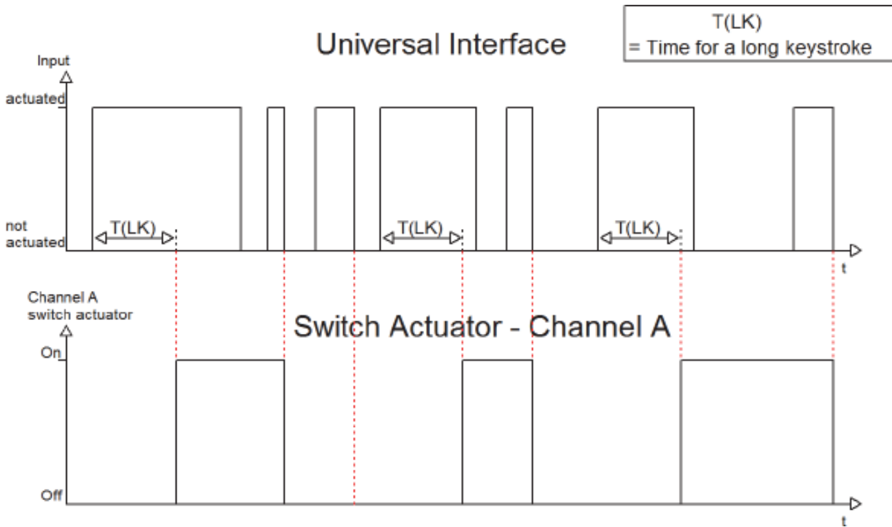
Picture 22: Long press / short press fit
