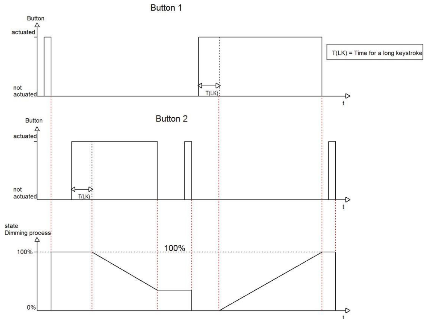
Picture 6: Double key dimming waveform
