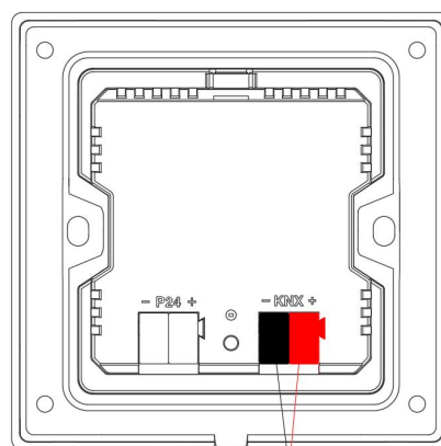
wiring diagram
